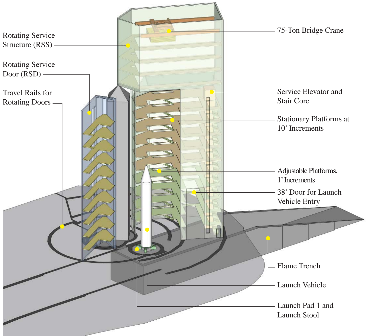
Kodiak Launch Complex Launch Service Structure and Launch Pad 1
